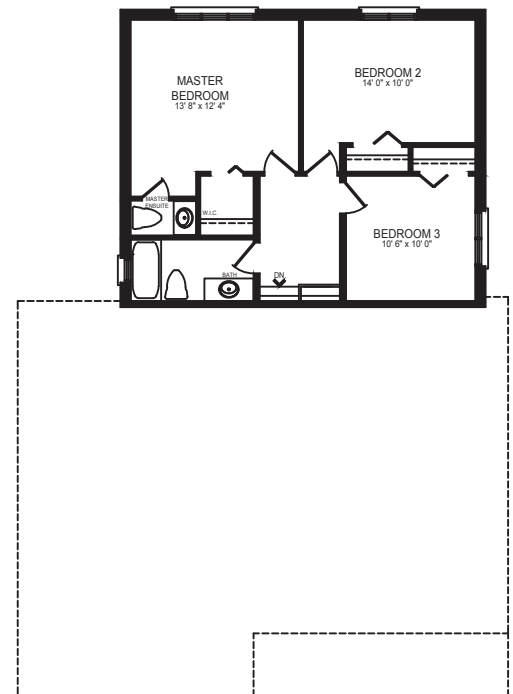
SECOND FLOOR PLAN APPROX. 715 SQ.FT.
