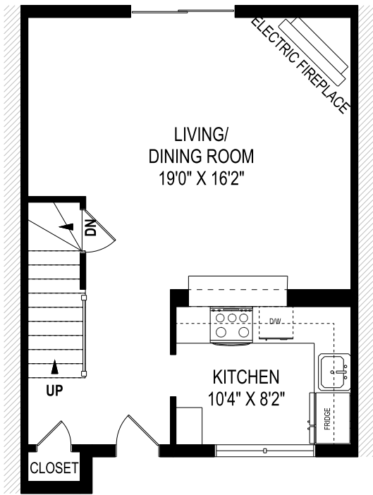
MAIN FLOOR PLAN 540 SQUARE FEET
