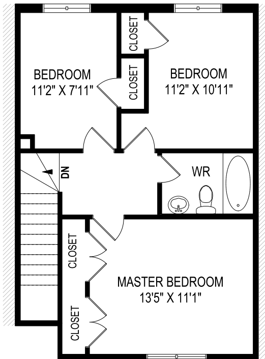
SECOND FLOOR PLAN 570 SQUARE FEET
